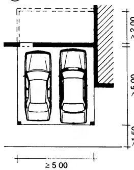
11 Two cars, room for bicycles
